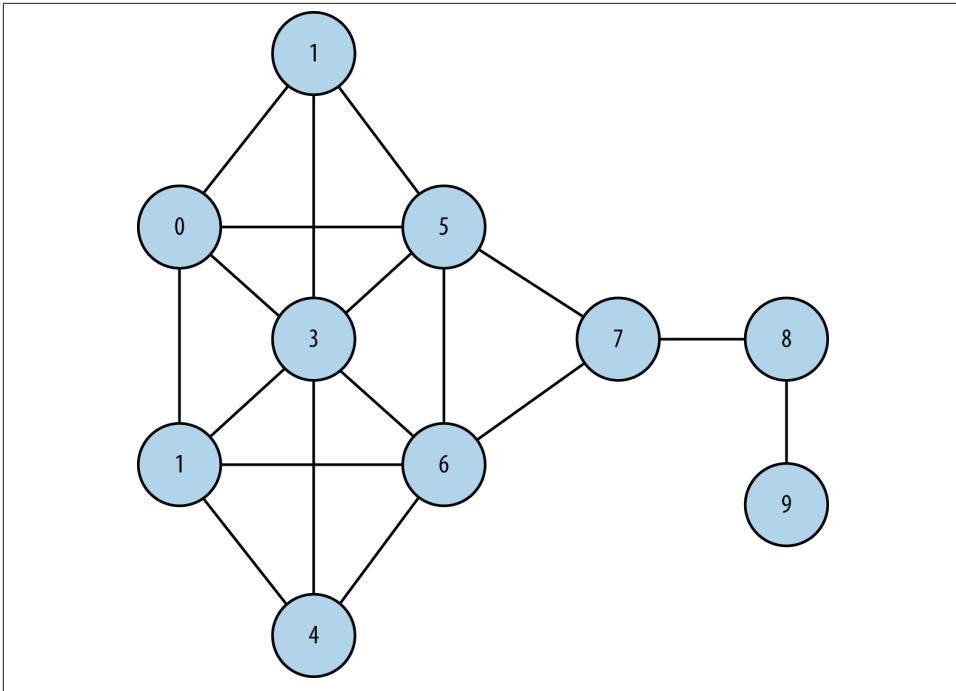
Figure 7-4. The Krackhardt kite graph that will be used to illustrate degree, betweenness, and closeness centrality measures
