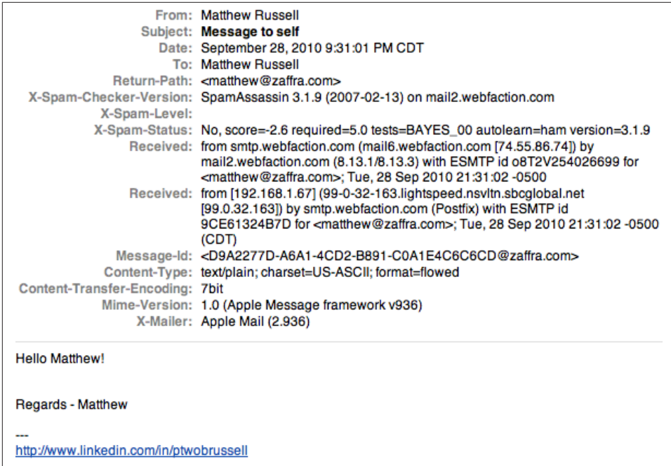
Figure 6-1. Most mail clients allow you to view the extended headers through an options menu
