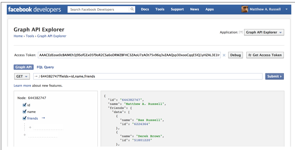
Figure 2-2. Using the Graph API Explorer application to progressively build up a query for friends' interests: a query for a node and connections to friends
